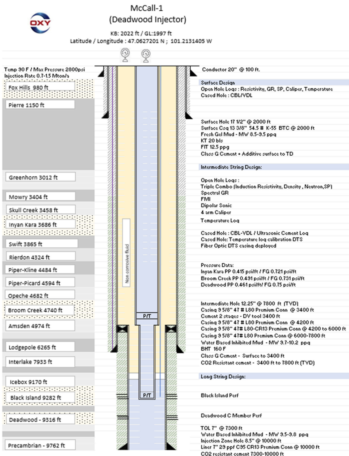
Figure 4-12. Proposed design of the McCall-1 Deadwood CO 2 injection wellbore schematic.
