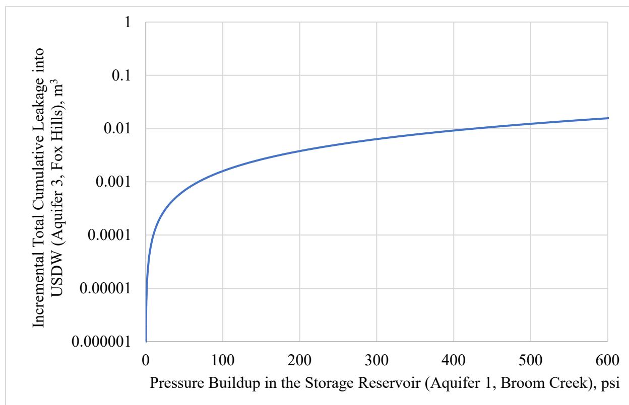
Figure A-22. Relationship between pressure buildup (x-axis, psi) in the storage reservoir (Aquifer 1, Broom Creek) and incremental total cumulative leakage (y-axis, m³) for Aquifer 3 (USDW, Fox Hills). In this scenario, the leaky wellbore is closed to Aquifer 2 (Inyan Kara).
