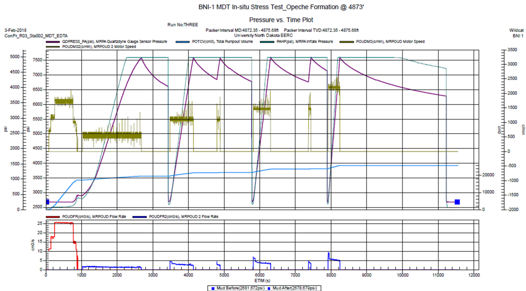
Figure 2-38. BNI-1 Opeche/Spearfish Formation MDT microfracture in situ stress pump cycle graph at 4,873 ft.
