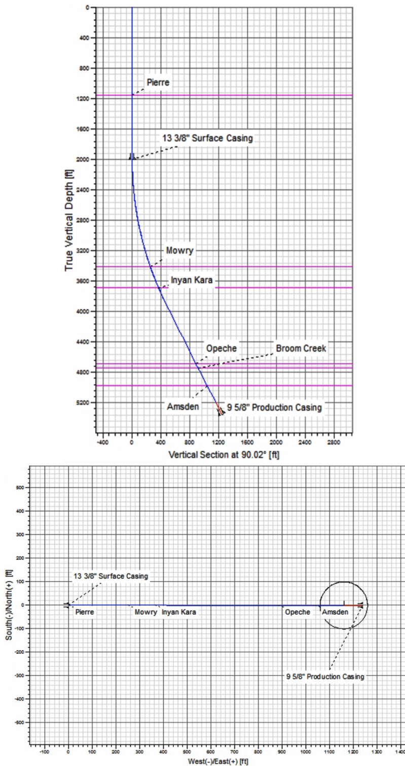
Figure 4-13. Unity-1 proposed well trajectory.
