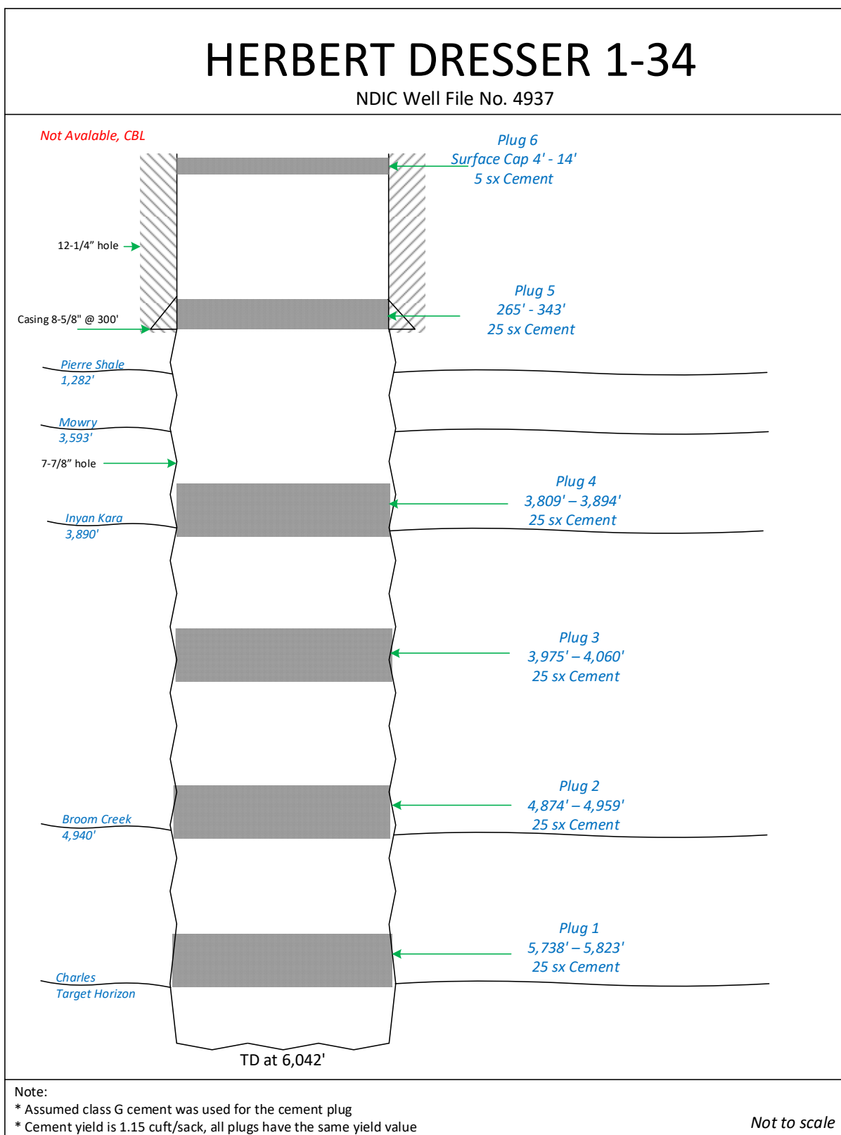
Figure 3-8. Herbert Dresser 1-34 (NDIC File No. 4937) well schematic showing the location and thickness of cement plugs.
