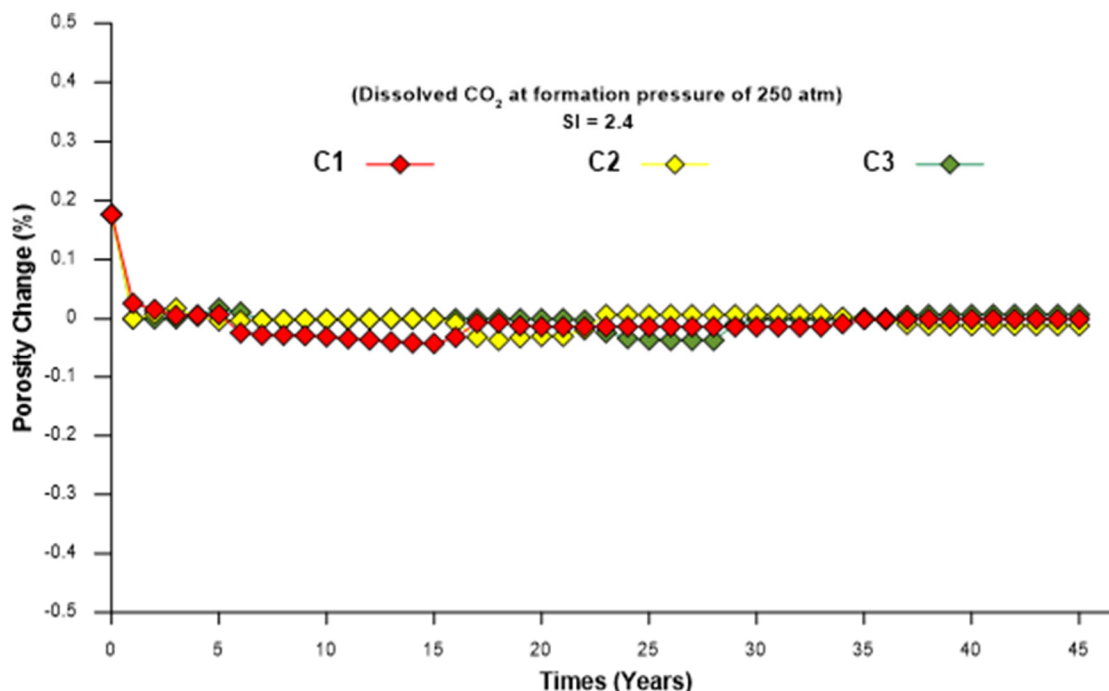
Figure 2-51. Change in percent porosity in the Amsden underlying confining layer red line shows porosity change for Cell C1, 0 to 1 meter below the Amsden top. Yellow line shows Cell C2, 1 to 2 meters below the Amsden top. Green line shows Cell C3, 2 to 3 meters below the Amsden top. Long-term change in porosity is minimal and stabilized. Positive change in porosity is related to precipitation of minerals, and negative change is due to mineral dissolution.
