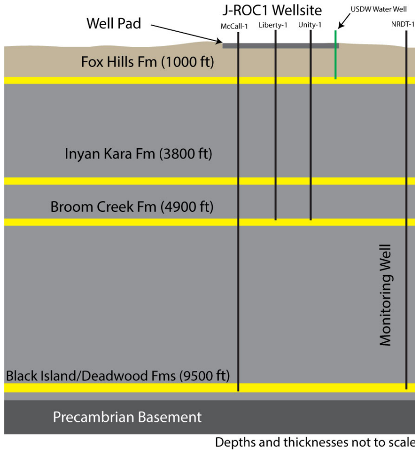
Figure 4-5. Monitoring schematic (not to scale) includes the location of the Broom Creek injectors (Liberty-1 [J-ROC1 File No. 37672] and Unity-1 [proposed]), the Deadwood injector (McCall-1 [proposed]), and the monitoring well NRDT-1 (proposed).
