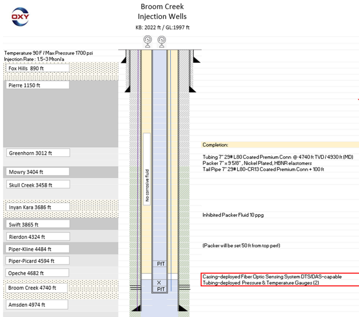
Figure 4-8. Broom Creek injection wellbore schematics showing placement of tubing-deployed pressure and temperature-monitoring gauges and casing-deployed fiber optic sensing system (DTS/DAS-capable).
