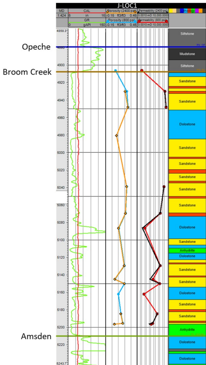
Figure 2-15. Vertical distribution of core-derived porosity and permeability values in the Tundra SGS CO 2 storage complex.
