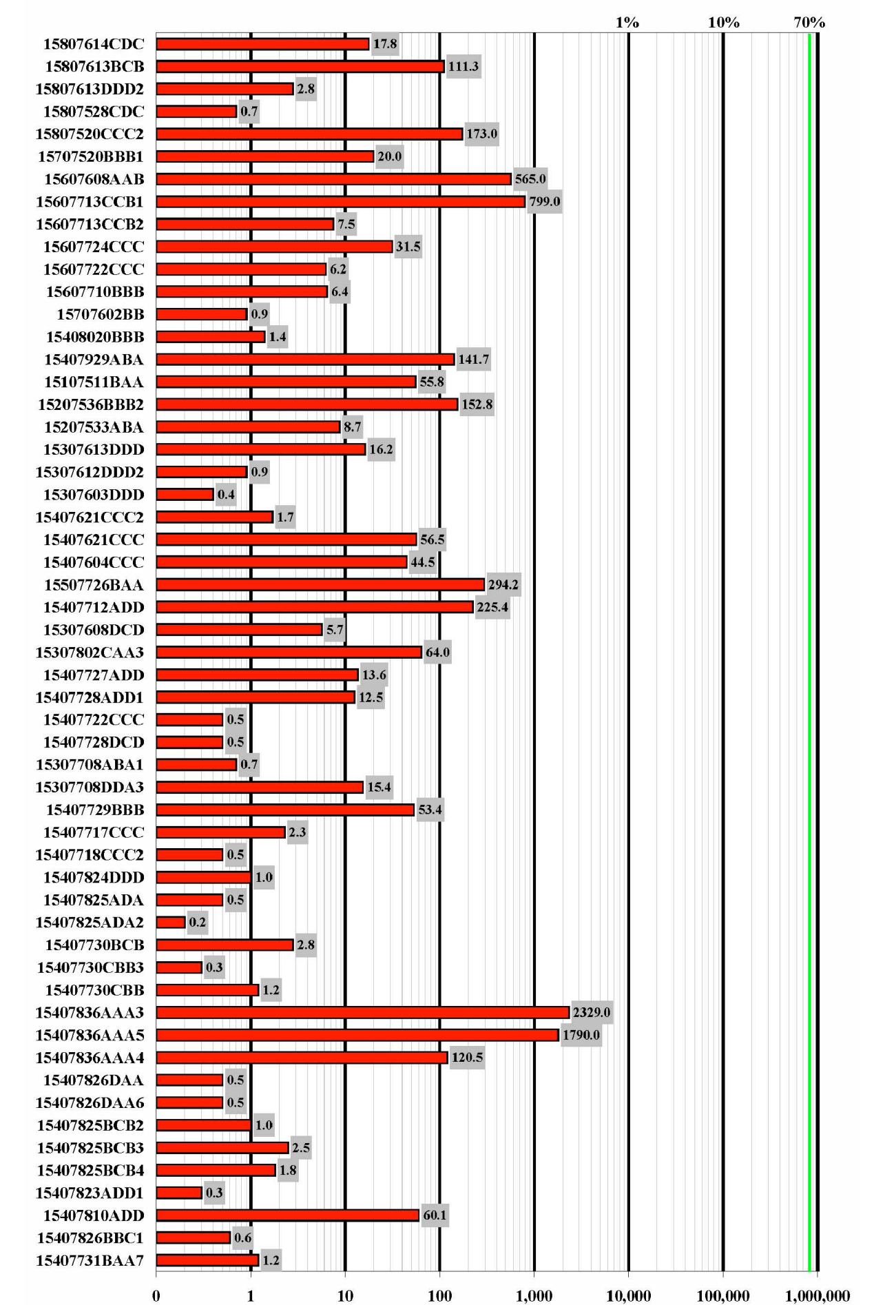
Figure 1. Graph depicting the relative relationship and maximum values of FID instrument responses from selected wells in McHenry County. FID results for each well are presented in order of sampling occurrence from top to bottom. Values shown are those reported from the ground-water/air interface (as CH 4 in ppm). The typical concentration of methane in commercial natural gas is highlighted by the vertical green line at 70%.
