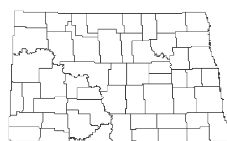
Zealand Quadrangle, North Dakota
