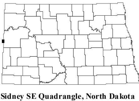
Sidney SE Quadrangle, North Dakota
