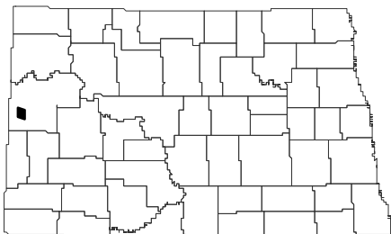
Sheep Creek Quadrangle, North Dakota
