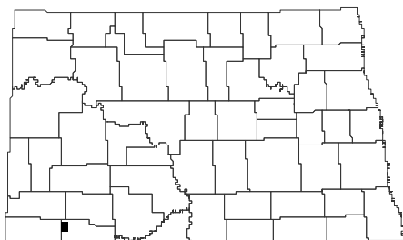
Whetstone Buttes Quadrangle, North Dakota
