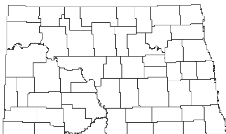
Cow Butte NE Quadrangle, North Dakota
