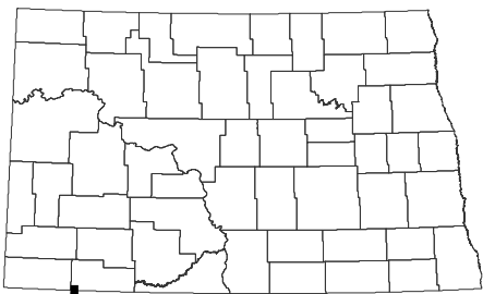
Cow Butte Quadrangle, North Dakota
