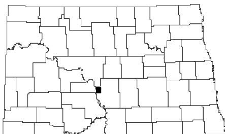
Wilton SE Quadrangle, North Dakota
