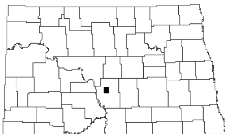
Regan SE Quadrangle, North Dakota
