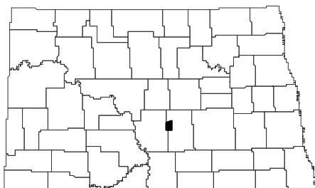
Harriet Lake SE Quadrangle, North Dakota
