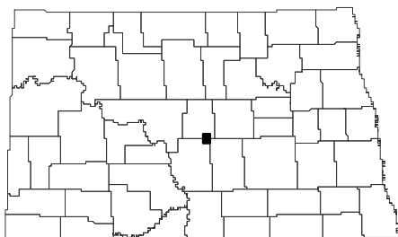
Goodrich SW Quadrangle, North Dakota
