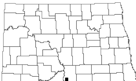
Kiefer Buttes Quadrangle, North Dakota
