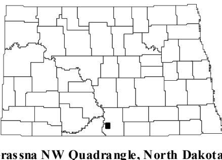
Grassna NW Quadrangle, North Dakota
