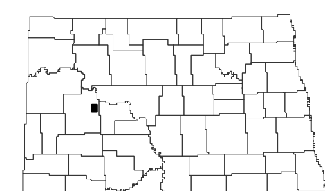
Halliday NE Quadrangle, North Dakota
