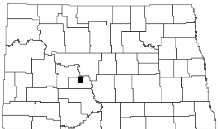
Hannover NE Quadrangle, North Dakota
