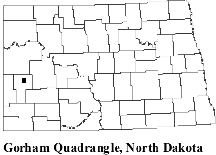
Gorham Quadrangle, North Dakota
