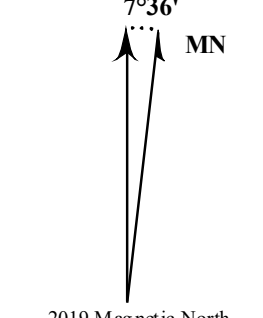
2019 Magnetic North Declination at Center of Sheet
