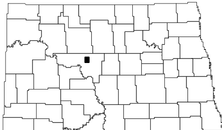
Coleharbor NW Quadrangle, North Dakota
