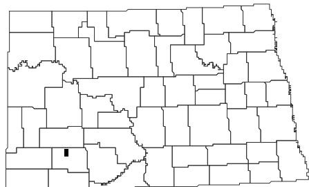
Stony Butte Quadrangle, North Dakota
