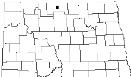
Landa SE Quadrangle, North Dakota
