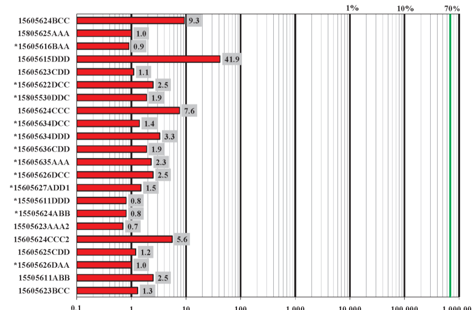
Figure 1. Graph depicting the relative relationship and absolute maximum values of flame-ionization detector (FID) instrument responses from selected wells in Walsh County. FID results for each well are presented in order of field screening occurrence from top to bottom. Values shown are those reported from the ground-water/air interface (GWI) (as CH 4 in ppm). The concentration of methane typical in commercial natural gas is highlighted by the vertical green line at 70%.
