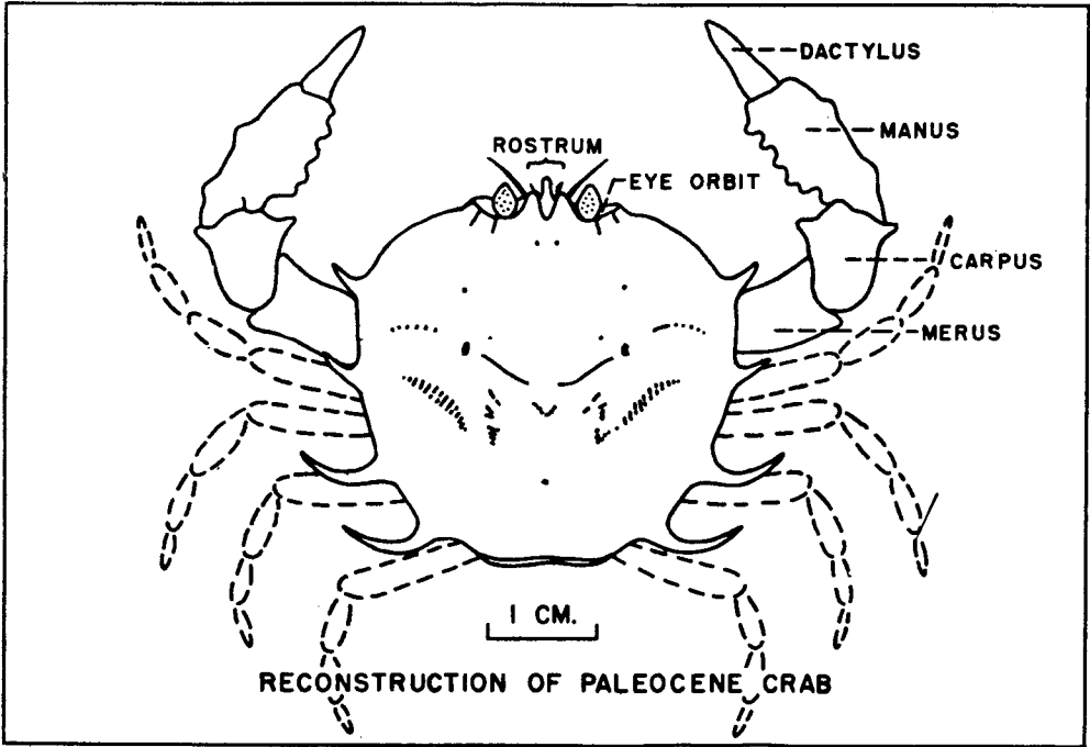
TEXT-FIG. 2—Diagrammatic scale reconstruction of Camarocarcinus arnesoni Holland & Cvanara, n. gen., n. sp. Dashed lines hypothetical and the eyes, antennae, and antennules are completely hypothetical. The merus (?) of one ambulatory leg is known, but it is more slender than any shown here. The carpi of the chelipeds are shown rotated rather too far inward and the meri are a bit heavy. The chelipeds were likely carried folded closely in against the front of the body. The round axial posterior dot indicates the position of the cardiac node; the other marks indicate indentations of the exoskeleton.
