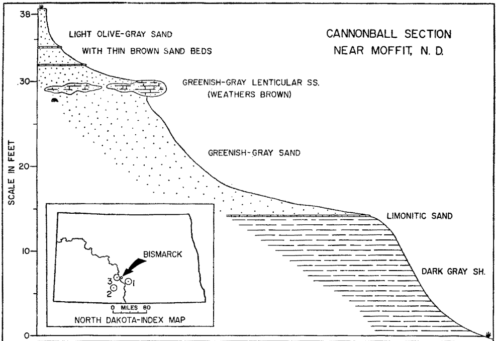
TEXT-FIG. 1.—Section of Paleocene Cannonball formation in road-ditch exposure, Locality No. 1, near Moffit, southern Burleigh County, North Dakota. This is the type locality of Camarocarcinus arnesoni Holland & Cvancara, n. gen. n. sp., and Ranina (?) burleighensis Holland, n. sp.; the crabs were found free, loose on the surface, mostly near the upper part (31 to 35 feet above base of measured section) of the exposure. The insert map shows the two principal areas where Camarocarcinus occurs (Locality 1a is only one mile west of Locality 1 and hence these two localities are covered by dot of No. 1).
