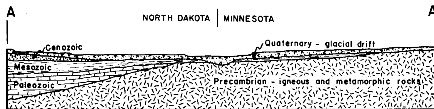
Figure 1. Physiographic map showing the location of Trail County. The cross-section A-A' shows the regional geologic relationships.
