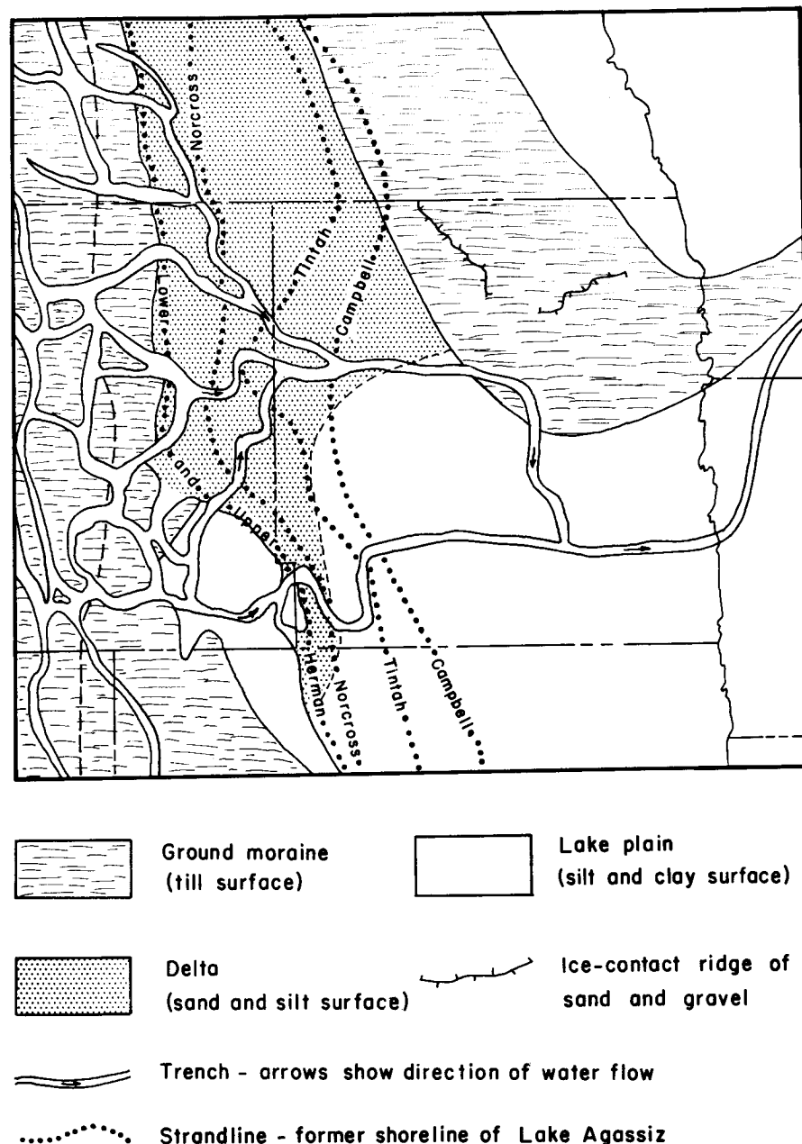
Figure 9. First draining of Lake Agassiz. When the ice receded far enough, an outlet was opened into the Superior basin and the lake drained, exposing the surface shown above. The Goose and Elm Rivers crossed Traill County (the Elm is the one on the south that enters Minnesota) cutting trenches in the lake sediments and depositing sand and gravel in those trenches.
