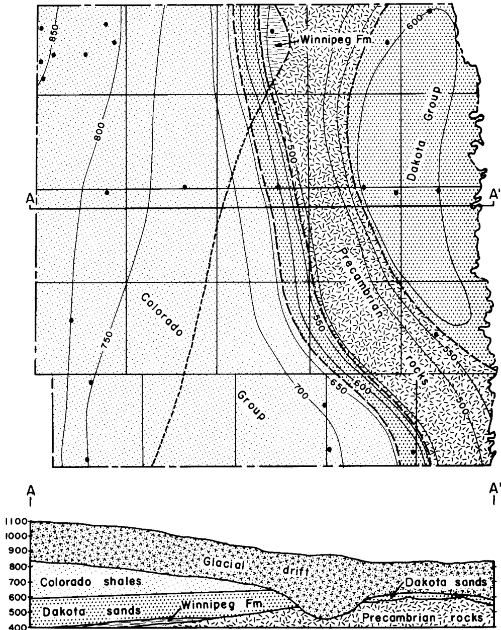
Figure 2. Topographic map of the bedrock surface beneath the glacial drift. Precambrian rocks subcrop beneath the drift in the valley, along with some Paleozoic Winnipeg shales in the northern part of the county. Colorado Group shales subcrop over the western half of the county; Dakota Group sands in the east. The approximate eastern limit of the Winnipeg shale beneath the Cretaceous sediments is shown as a dashed line.
