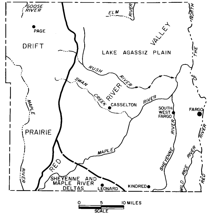
FIGURE 3. Physiographic divisions and drainage.
