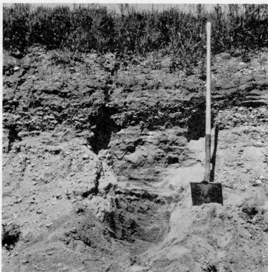
FIGURE 15. Typical beach deposit in SW1/4 sec. 1, T. 141 N., R. 53 W. View of Tintah beach looking west.
