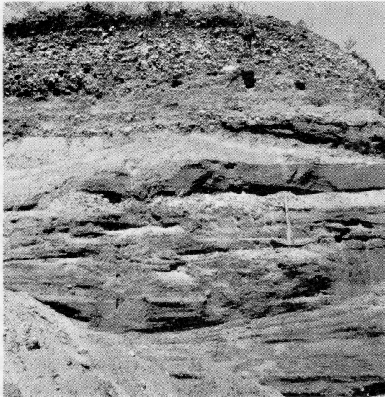
FIGURE 14. Stratified sand and gravel in terrace deposit, east side of Maple River in NW1/4 sec. 15, T. 138 N., R. 55 W.
