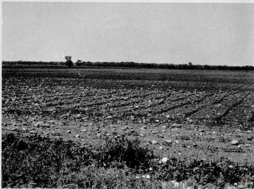
Figure 23. Concentration of cobbles in a field in the Lake Agassiz plain north of Wahpeton. SE \frac{1}{4} sec. 18, T. 133 N., R. 47 W.
