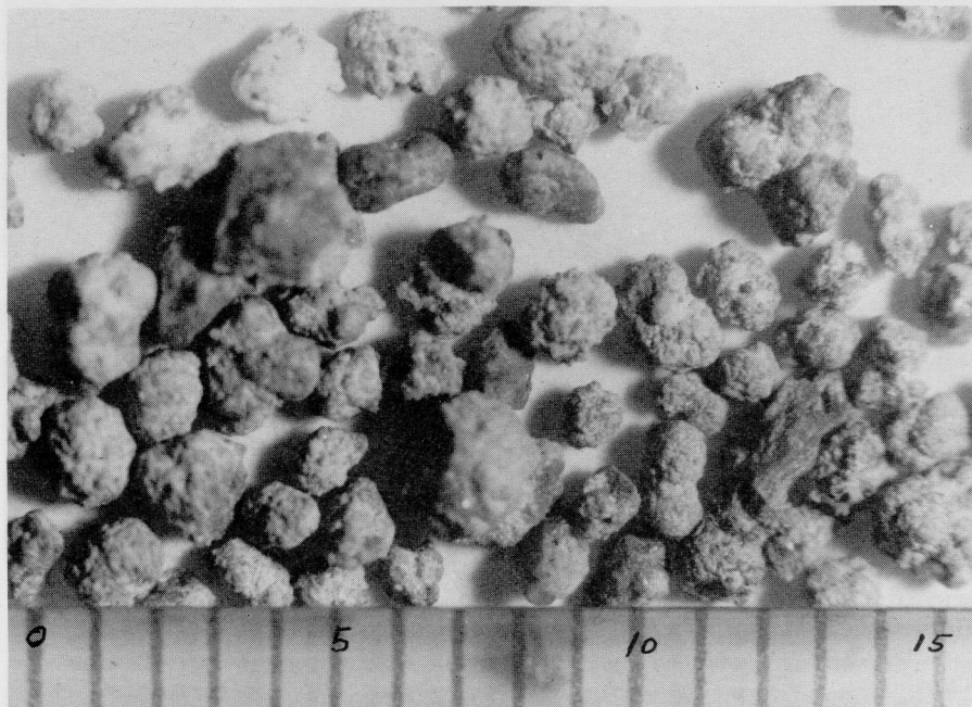
Figure 5. "Nodular" sand. Sample from test hole 3170, 131-52-25ccc; depth about 630 feet. Scale in millimeters.
