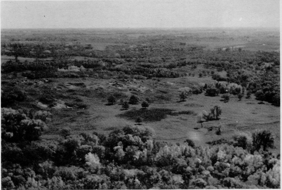
Figure 18. Dunes on the Sheyenne delta. View looking east toward the Lake Agassiz plain from near center of T. 136 N., R. 51 W. Oblique airphoto.
