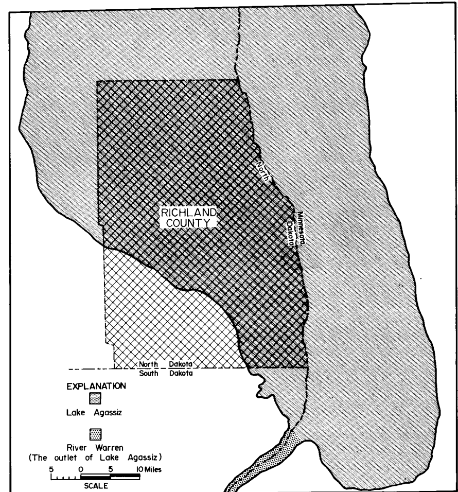
Figure 3. South end and outlet of Lake Agassiz during the highest stage of the lake.
