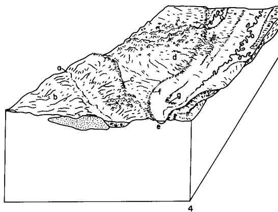
4. Lake Agassiz has receded completely from Richland County. The Sheyenne River is deeply entrenched in the delta, and high dunes are forming near the river valley. The axis of the lake bed is occupied by the Red River of the North and the Bois de Sioux River. The land forms are essentially as seen today. c-Herman beach, f-Campbell beach, g-McCauleyville beach.
