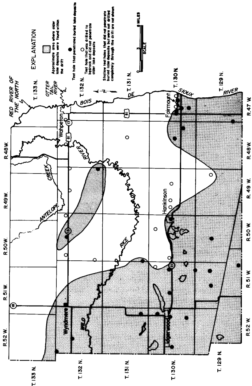
Figure 9. Location of buried lake deposits in southern Richland County.
