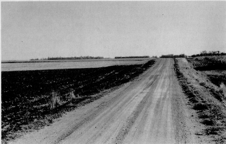
Figure 21. The Herman beach south of Wyndmere. Change in slope of the road marks the beach front. View looking south from the Lake Agassiz basin. Road marks line between secs. 4 and 5, T. 131 N., R. 51 W.
