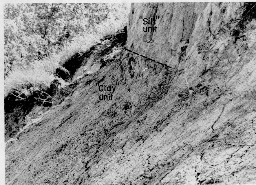
Figure 24. Exposure of two lithologic units of Lake Agassiz deposits in the bank of the Red River. SW \frac{1}{4} sec. 29, T. 135 N., R. 48 W.
