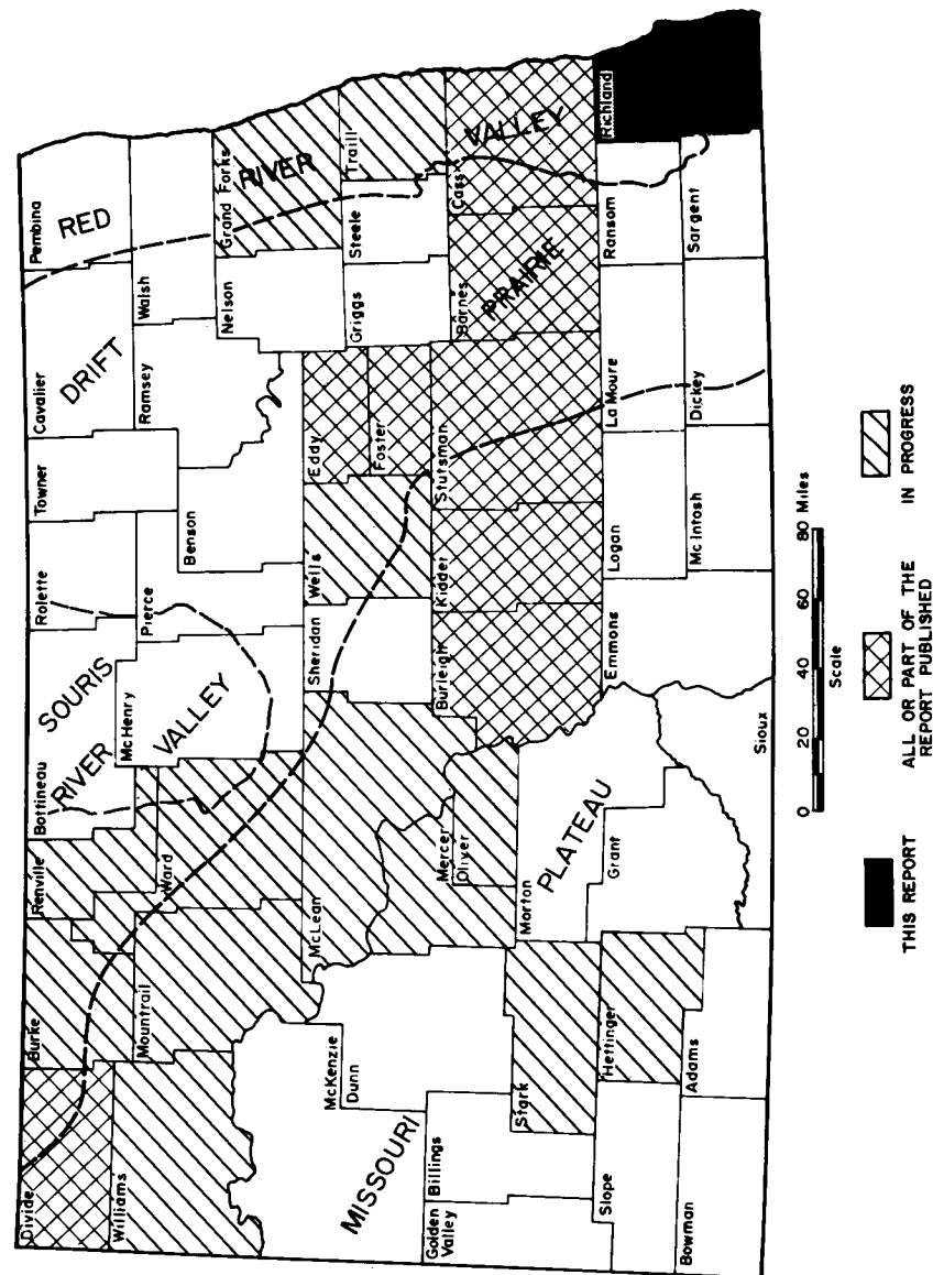
Figure 1. Physiographic divisions and locations of county ground-water studies.
