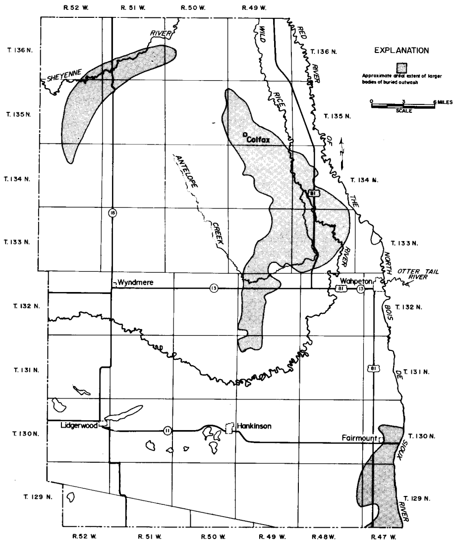
Figure 8. Approximate location of larger bodies of buried outwash.
