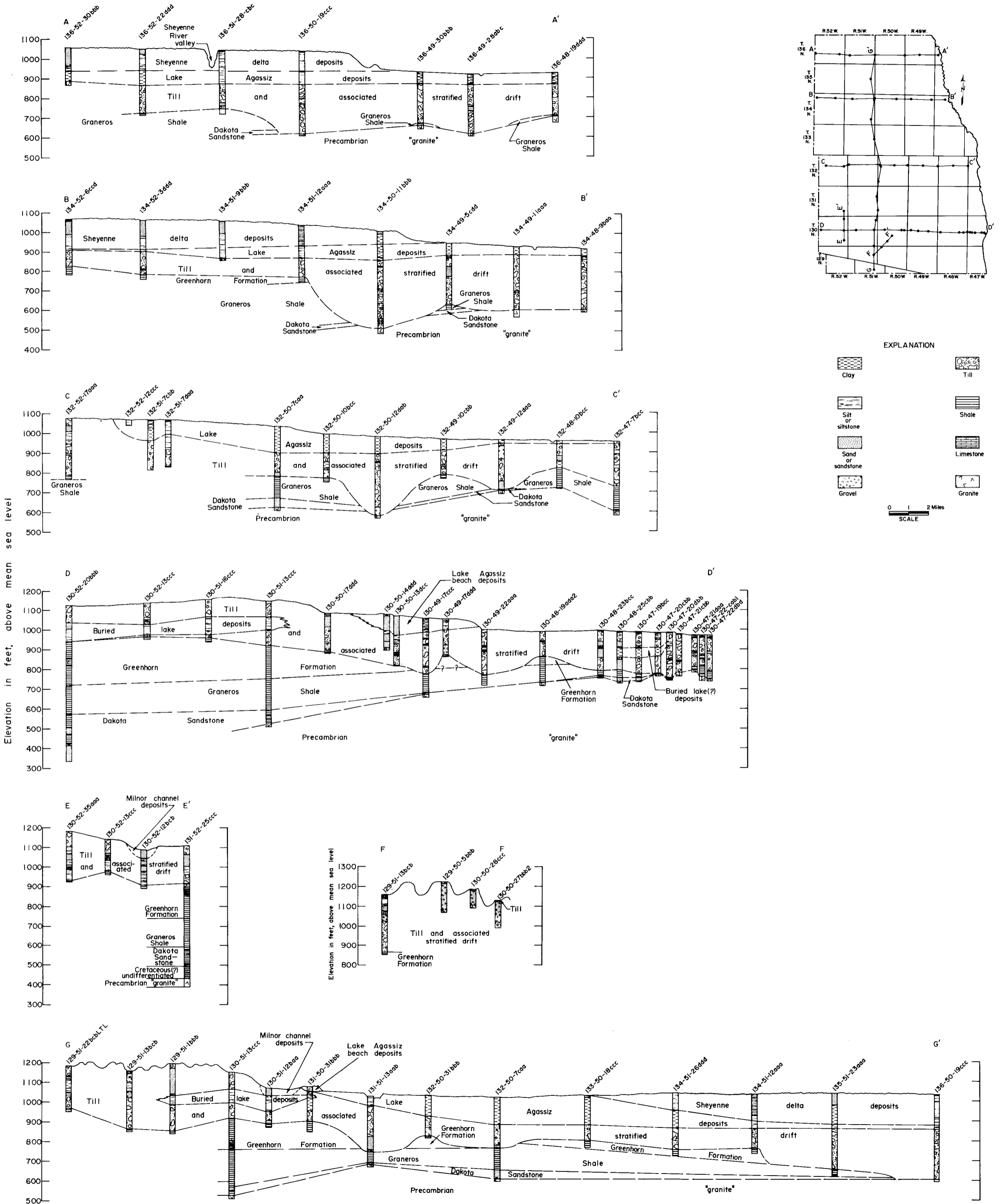
PLATE 4. Geologic sections in Richland County, N. Dak.
