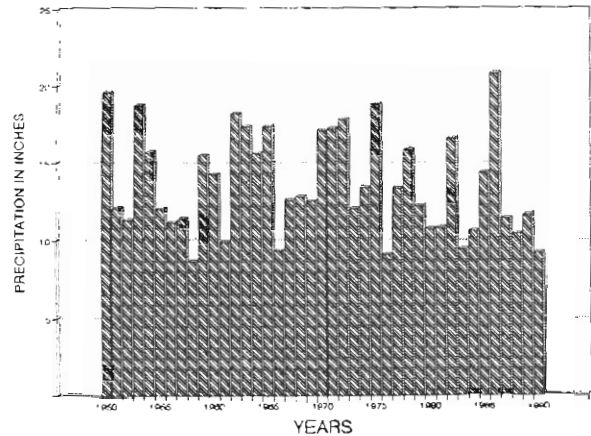
Figure 63. Annual precipitation at Williston from 1950-1990.
