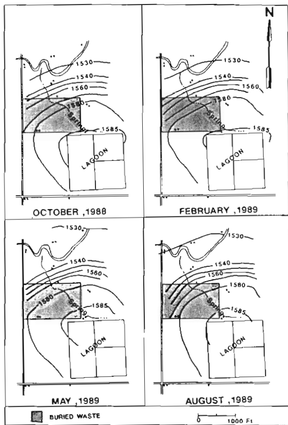
Figure 35. Water table maps for the Harvey landfill.
