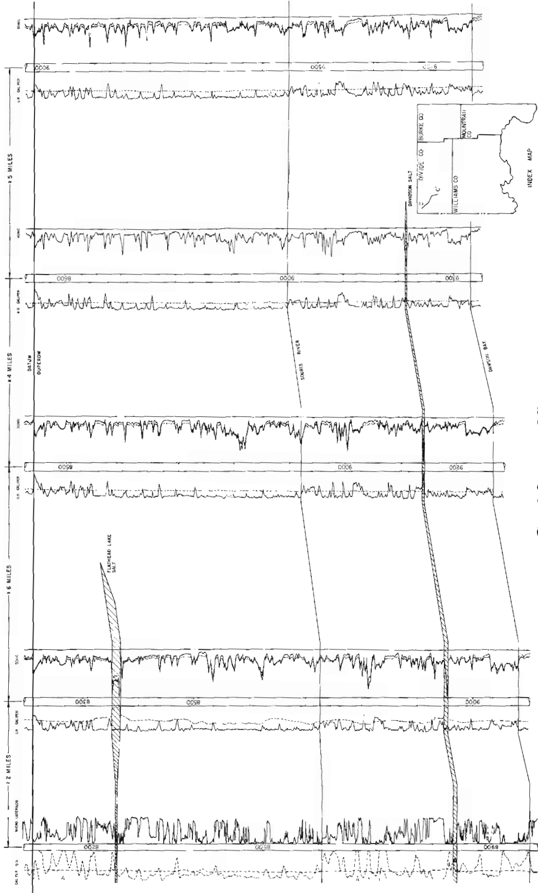
Figure 8. Cross section C-C'.
