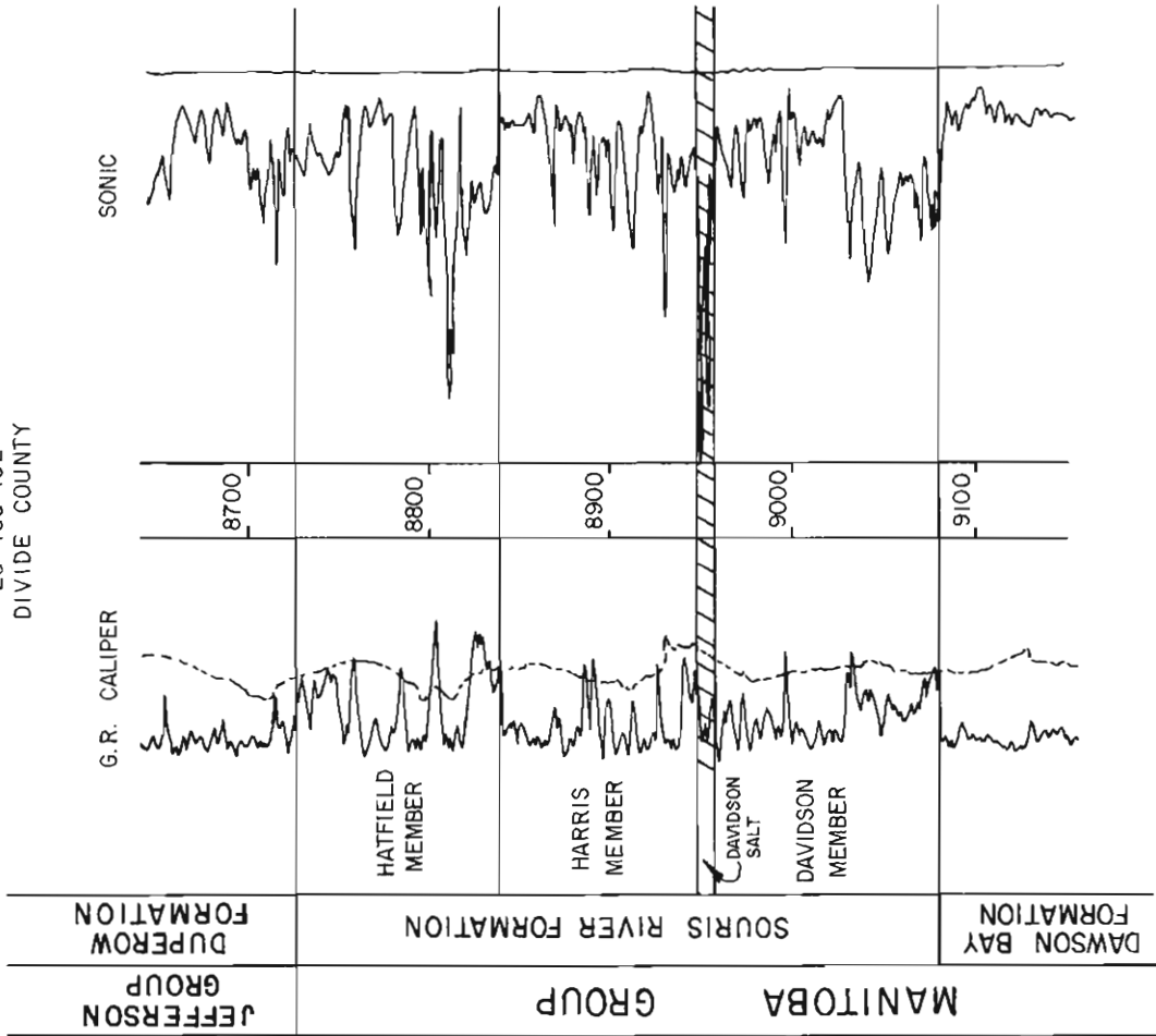
Figure 11. Log character: Davidson Salt, Souris River Formation.
