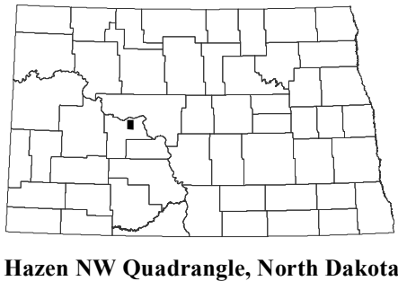
Hazen NW Quadrangle, North Dakota
