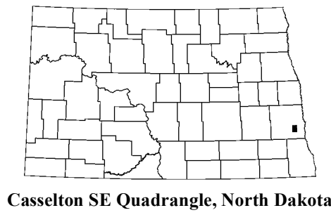
Casselton SE Quadrangle, North Dakota
