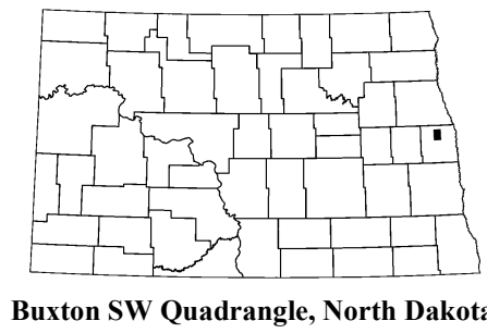
Buxton SW Quadrangle, North Dakota
