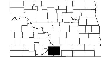
Linton 100K Sheet, North Dakota
