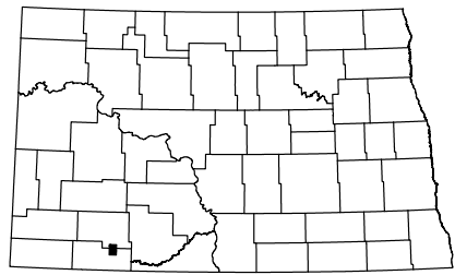
Long Butte Quadrangle, North Dakota
