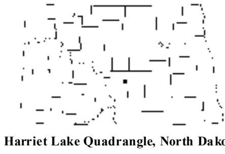
Harriet Lake Quadrangle, North Dakota
