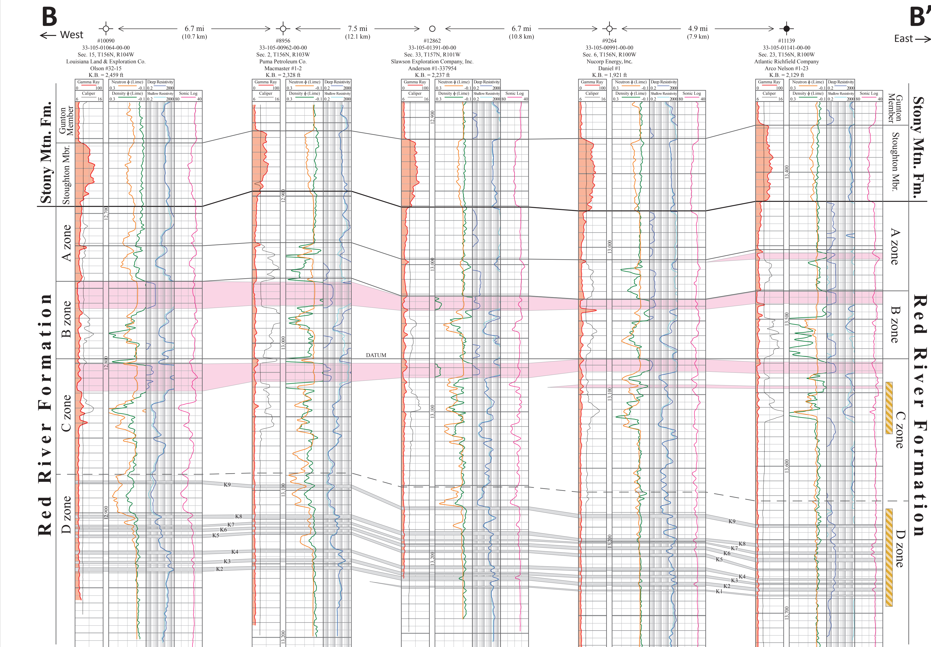
Figure 2: East-west cross-section of the upper Red River Formation displaying correlations of zones A-D tops, anhydrite beds, and kukersite intervals across western North Dakota. Anhydrite beds are correlated with light pink and kukersite beds are correlated with light gray. Less certain anhydrite and kukersite correlations are indicated by alternating pink/gray and white coloration. The formal (Stoughton Member - Stony Mountain Formation) and informal (A-D zones - Red River Formation) member tops are displayed by solid thin black lines while the approximate Red River D zone is displayed as a dashed line. The cross-section datum is the top of the Red River C zone. Wireline log depths are in feet and represent true vertical depths from surface (Kelly bushing) elevation. Brown rectangles with diagonal lines represent Red River Formation core intervals. Well information is listed above each wireline log set, including in descending order: North Dakota Industrial Commission well number, API well number, section-township-range, original operator, original well name, and Kelly bushing elevation. Fm. = Formation; ft. = feet; mi. = miles; K.B. = Kelly Bushing; km = kilometers; Mtn. = Mountain; ♯ = porosity.
