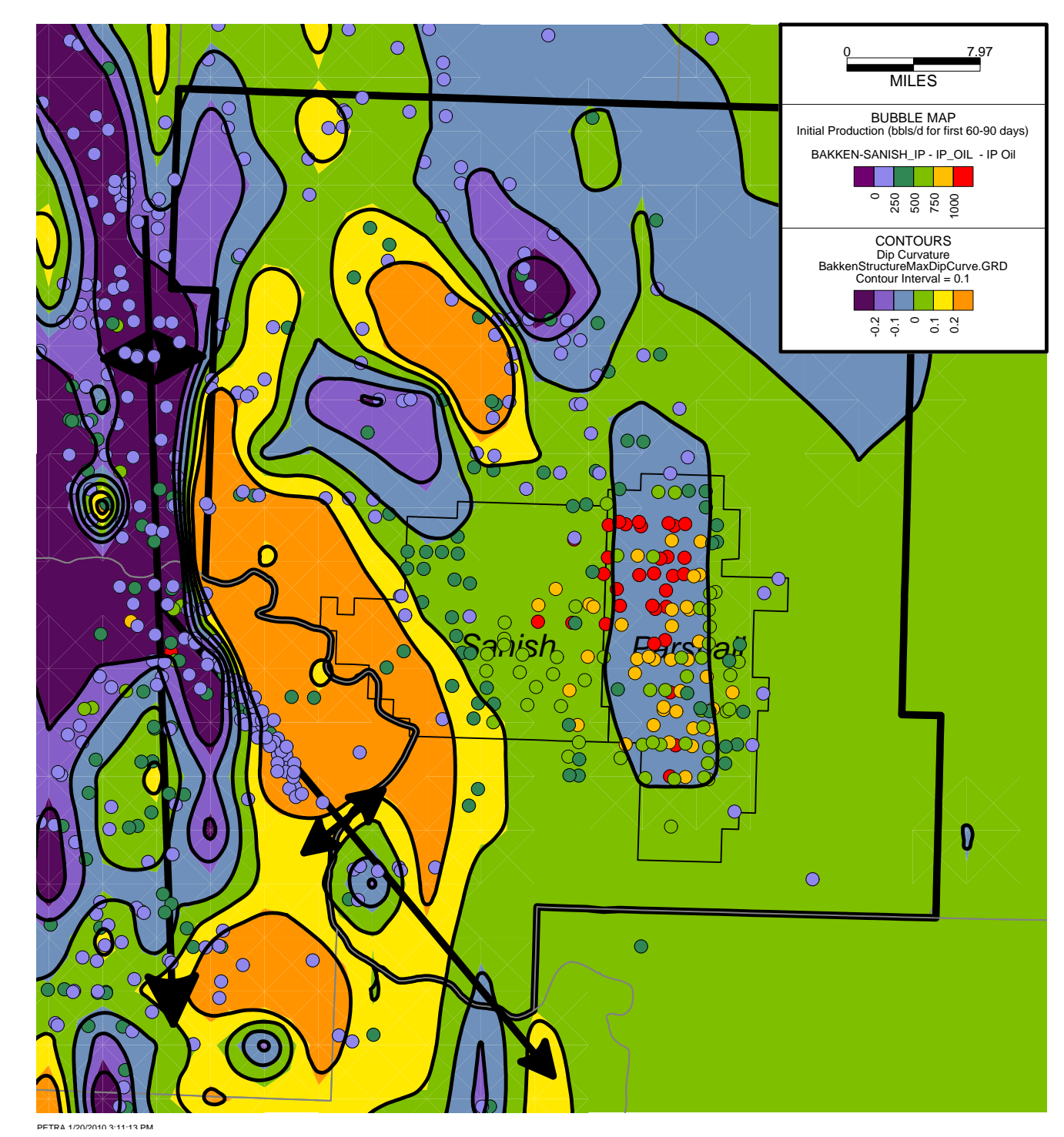
Figure 4. A dip curvature (2nd derivative) map constructed from the structure drawn on the top of the Bakken Formation. The contours of this map show the sense and degree of flexure that is present in the structure of the Bakken Formation in Mountrail County, ND. The map includes the approximate axis of the north-south trending Nesson Anticline and the southeastwardly plunging Antelope Anticline. The circles show the location of wells producing from the Bakken/Sanish pools with the fill color of the circle representing the average daily production (bbls/day) for the first 60 to 90 days of pumping.
