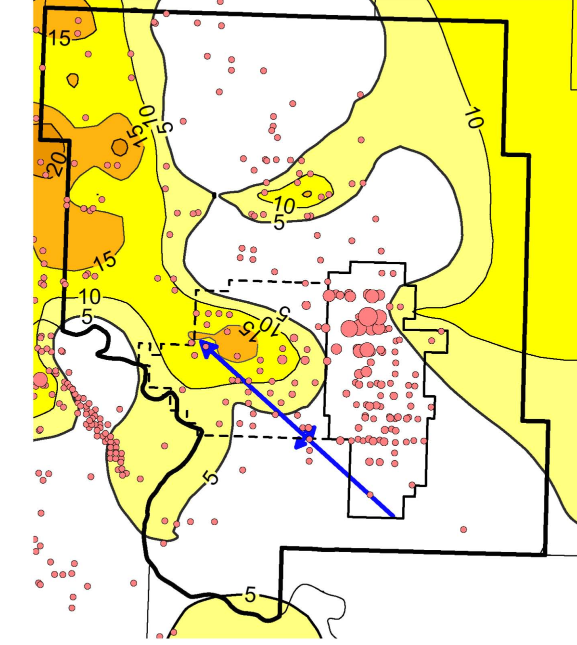
Figure 4 An isopach of Lithofacies 3 showing an updip pinch-out of the unit. The shaded intervals areas in which L3 is at least 5 ft thick. Each color change represent a 5 ft increase in thickness. Production levels in the county are plotted as circles with the radius being proportional to the daily average of the first 60 days of production.
