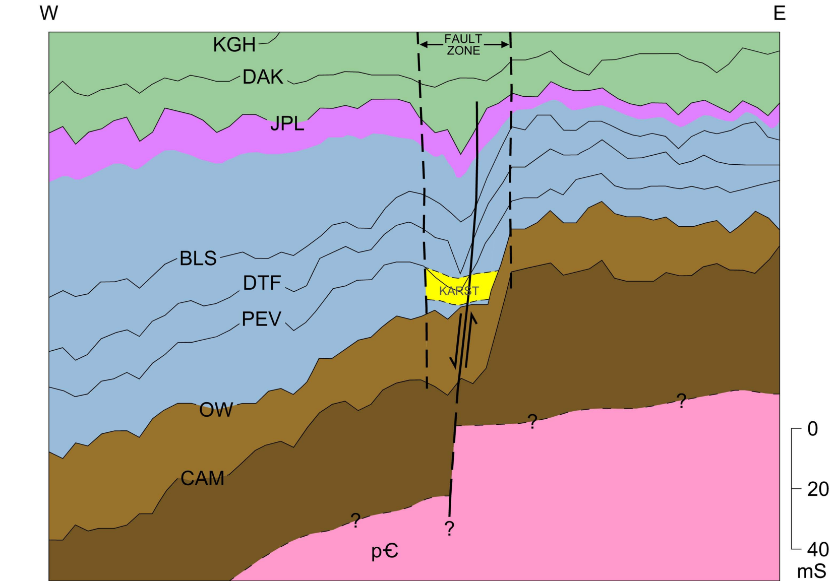
Figure 6. Interpreted seismic section showing the two way travel times for 7 reflectors in Mountrail County. The times are "hung" on the Greenhorn (KGH) reflector and show a prominent change in reflector dip when the vertical scale is exaggerated approximately 40 times. The tops portrayed include reflectors on the Dakota Formation (DAK), Piper Limestone (JPL), Base of the Last Salt (BLS), Three Forks (DTF), Prairie Evaporite (PEV), Winnipeg (OW) and the "Cambrian" (CAM). The maximum 2 way travel time displacement across the fault is on the order of 20 msec, which for a limestone (P-velocity ~ 6,000 ft/sec) translates to a physical displacement of about 60 ft. The structure on the Precambrian (pC) is inferred from the displacements apparent in the overlying section.
