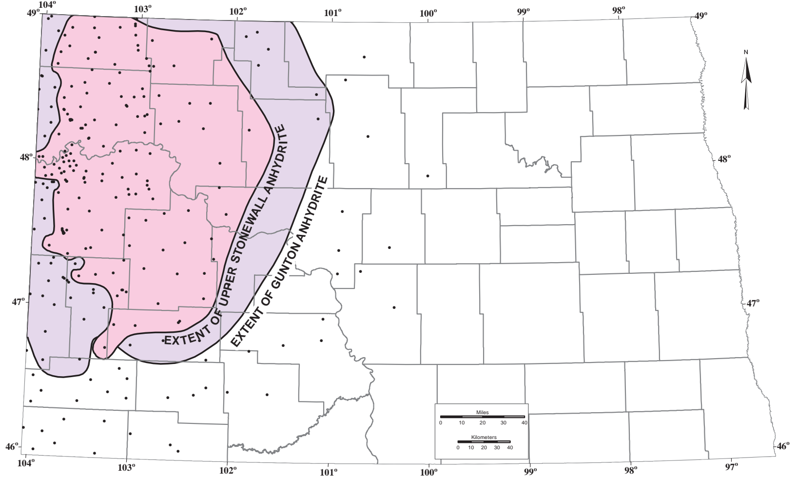
Figure 5 Map depicting the extent of the upper Stonewall and Gunton anhydrite intervals (Plate I). Black dots represent control wells. Wireline log examples of both anhydrite intervals are displayed on the Plate I cross-section.
