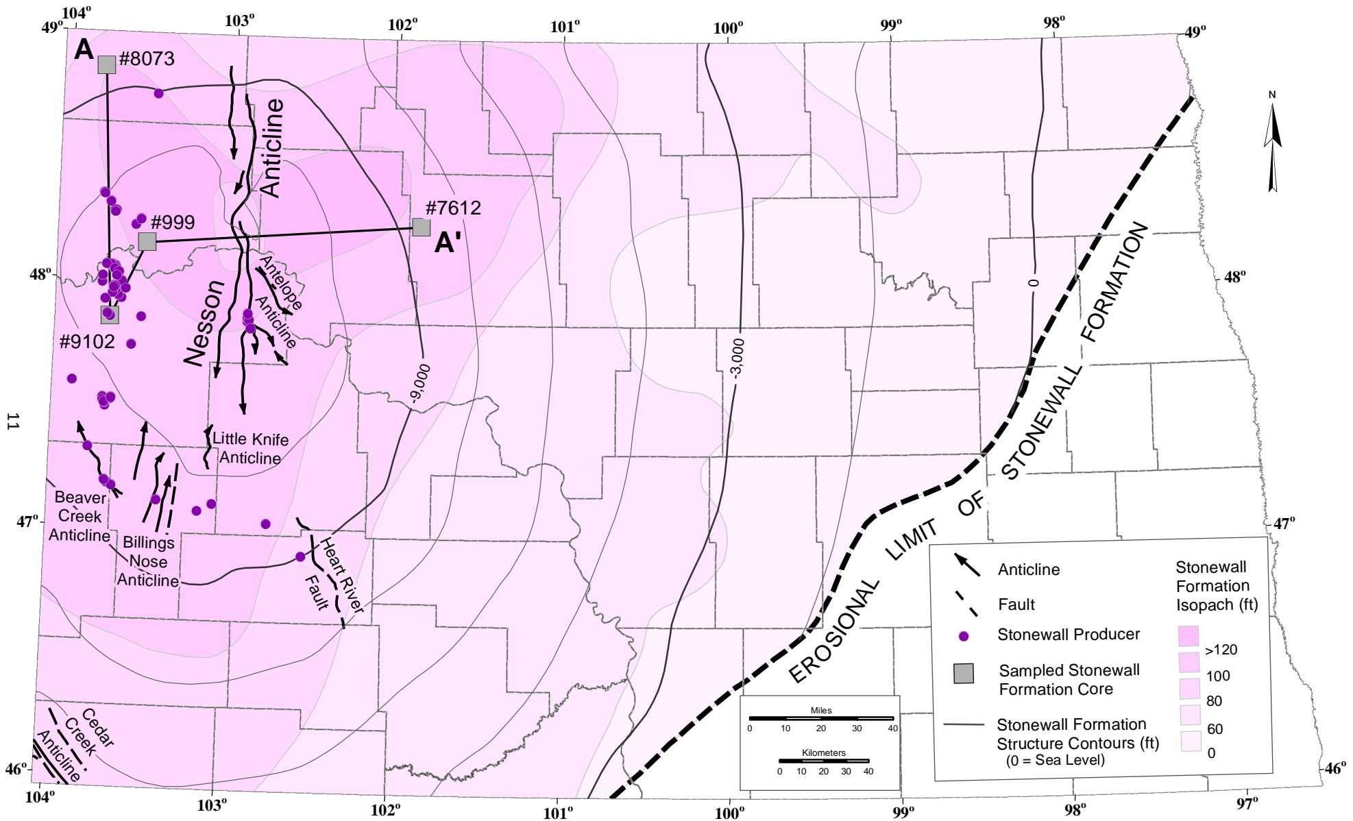
Figure 1. Map depicting the extent of the Stonewall Formation in North Dakota (colored area) and wells that have produced oil and gas from the Stonewall Formation (Carlson and Eastwood, 1962). A-A' indicates the location and orientation of the Plate 1 cross-section.
