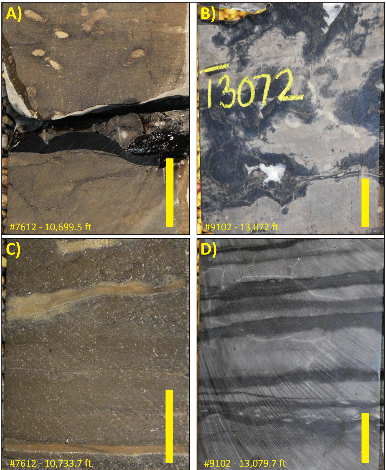
Figure 2. Core photograph examples from sampled Stonewall Formation cores. A) Dark brown dolomite mudstone (0.56-1.12% TOC) containing a black, highly organic-rich mudstone lamination (13.4% TOC, 102.7 mg/g S 2 ), B) tan and very dark grey/black, burrow mottled, dolomite mudstone (TOC: 0.65-2.56%), C) dark brown, laminated, lime mudstone (0.55-0.60% TOC), and D) grey to very dark grey, laminated, lime mudstone (0.06-0.22% TOC). The NDIC well number and approximate core depth of each sample is listed in bottom left hand corner of each photograph. Each thick yellow line represents 1 inch.
