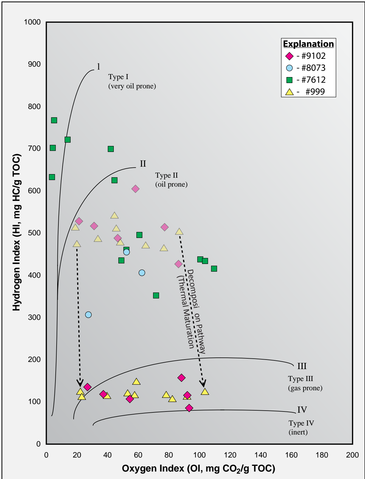
Figure 4. Modified Van Krevelen diagram depicting geochemical data from Stonewall Formation core samples as related to kerogen type/s. The semi-transparent symbols represent the estimated original HI and OI values of Stonewall core samples from the J. M. Donahue #1 (#999) and Gajewski #1-2-1A (#9102) cores.
