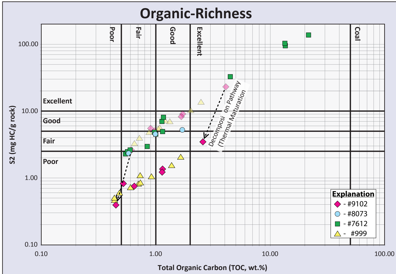
Figure 3. Organic-richness plot (Dembicki, 2009) of Stonewall Formation core samples. The semi-transparent symbols represent the estimated original organic-richness of samples from the J. M. Donahue #1 (#999) and Gajewski #1-2-1A (#9102) cores assuming 85% conversion of S2 (kerogen) into hydrocarbons.
